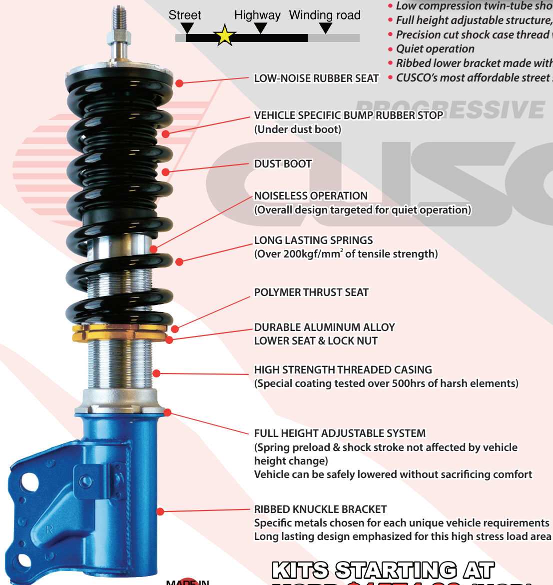
Pillowball Upper Mount Equipped Versions Available
